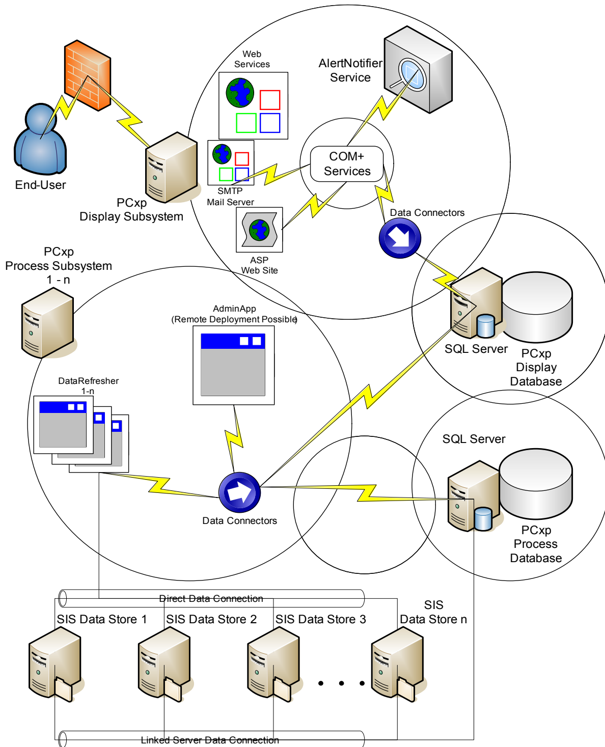
Figure 2-1. ParentCONNECTxp system
